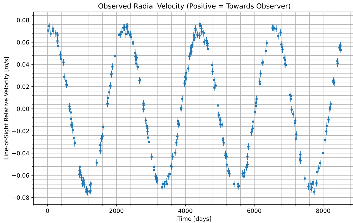
Figure 1: We have isolated the radial velocity of the host star due to the candidate planet. Data begins at UTC 2054-06-18/10:00. Positive values indicate the velocity at which the star is moving towards us; negative indicate the velocity at which it is moving away.
