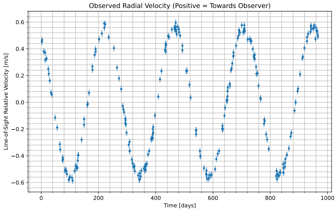
Figure 1: We have isolated the radial velocity of the host star due to the candidate planet. Data begins at UTC 2073-08-31/04:16. Positive values indicate the velocity at which the star is moving towards us; negative indicate the velocity at which it is moving away.
