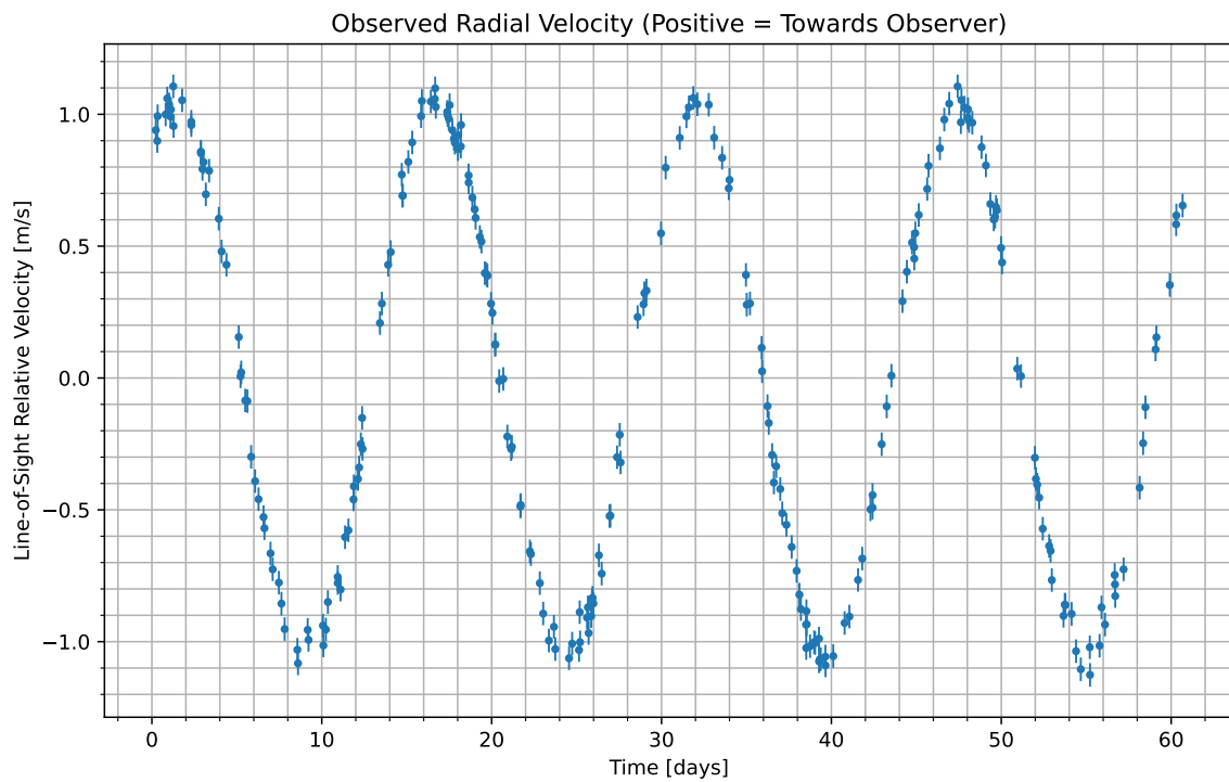
Figure 1: We have isolated the radial velocity of the host star due to the candidate planet. Data begins at UTC 2075-11-10/02:28. Positive values indicate the velocity at which the star is moving towards us; negative indicate the velocity at which it is moving away.
