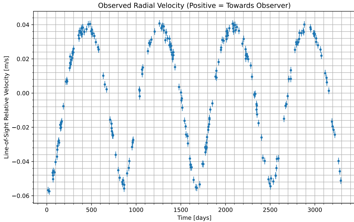
Figure 1: We have isolated the radial velocity of the host star due to the candidate planet. Data begins at UTC 2069-04-29/08:18. Positive values indicate the velocity at which the star is moving towards us; negative indicate the velocity at which it is moving away.
