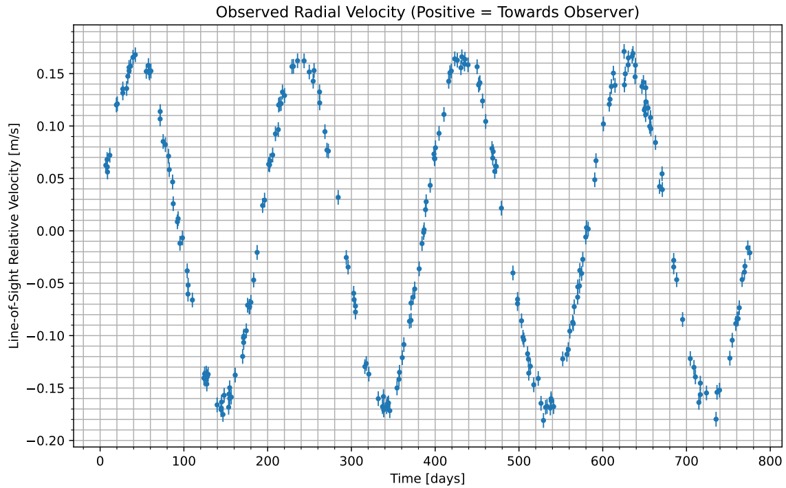
Figure 1: We have isolated the radial velocity of the host star due to the candidate planet. Data begins at UTC 2085-12-26/12:36. Positive values indicate the velocity at which the star is moving towards us; negative indicate the velocity at which it is moving away.
