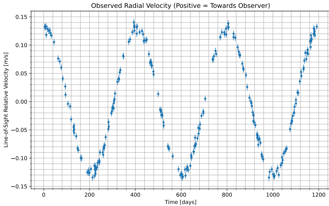
Figure 1: We have isolated the radial velocity of the host star due to the candidate planet. Data begins at UTC 2066-12-18/16:55. Positive values indicate the velocity at which the star is moving towards us; negative indicate the velocity at which it is moving away.
