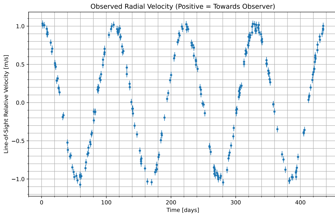
Figure 1: We have isolated the radial velocity of the host star due to the candidate planet. Data begins at UTC 2071-09-14/00:25. Positive values indicate the velocity at which the star is moving towards us; negative indicate the velocity at which it is moving away.
