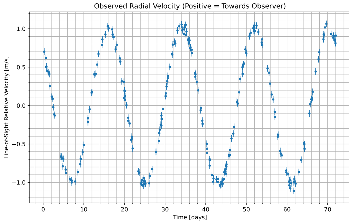
Figure 1: We have isolated the radial velocity of the host star due to the candidate planet. Data begins at UTC 2095-11-10/22:13. Positive values indicate the velocity at which the star is moving towards us; negative indicate the velocity at which it is moving away.
