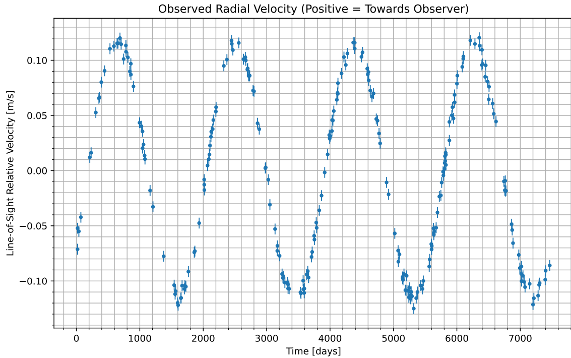
Figure 1: We have isolated the radial velocity of the host star due to the candidate planet. Data begins at UTC 2075-02-12/22:18. Positive values indicate the velocity at which the star is moving towards us; negative indicate the velocity at which it is moving away.
