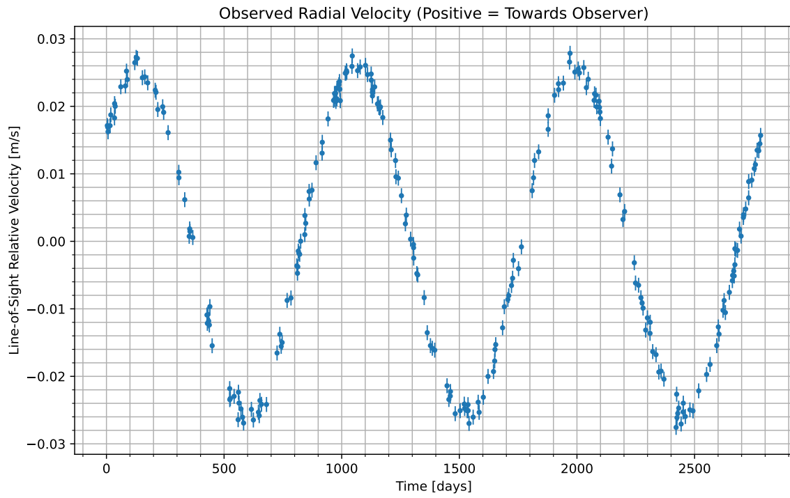
Figure 1: We have isolated the radial velocity of the host star due to the candidate planet. Data begins at UTC 2083-06-25/05:13. Positive values indicate the velocity at which the star is moving towards us; negative indicate the velocity at which it is moving away.
