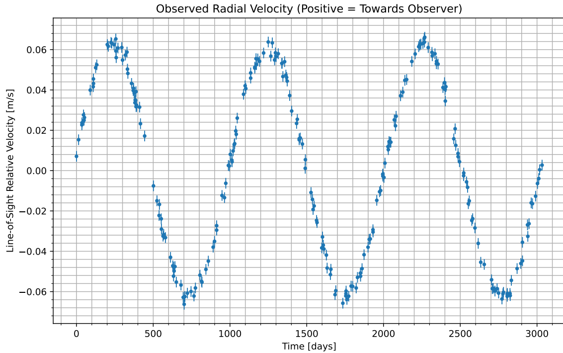
Figure 1: We have isolated the radial velocity of the host star due to the candidate planet. Data begins at UTC 2083-12-19/02:44. Positive values indicate the velocity at which the star is moving towards us; negative indicate the velocity at which it is moving away.
