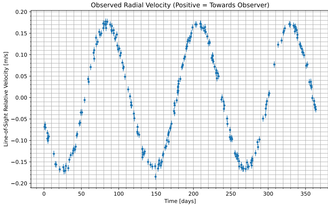
Figure 1: We have isolated the radial velocity of the host star due to the candidate planet. Data begins at UTC 2096-01-15/17:36. Positive values indicate the velocity at which the star is moving towards us; negative indicate the velocity at which it is moving away.
