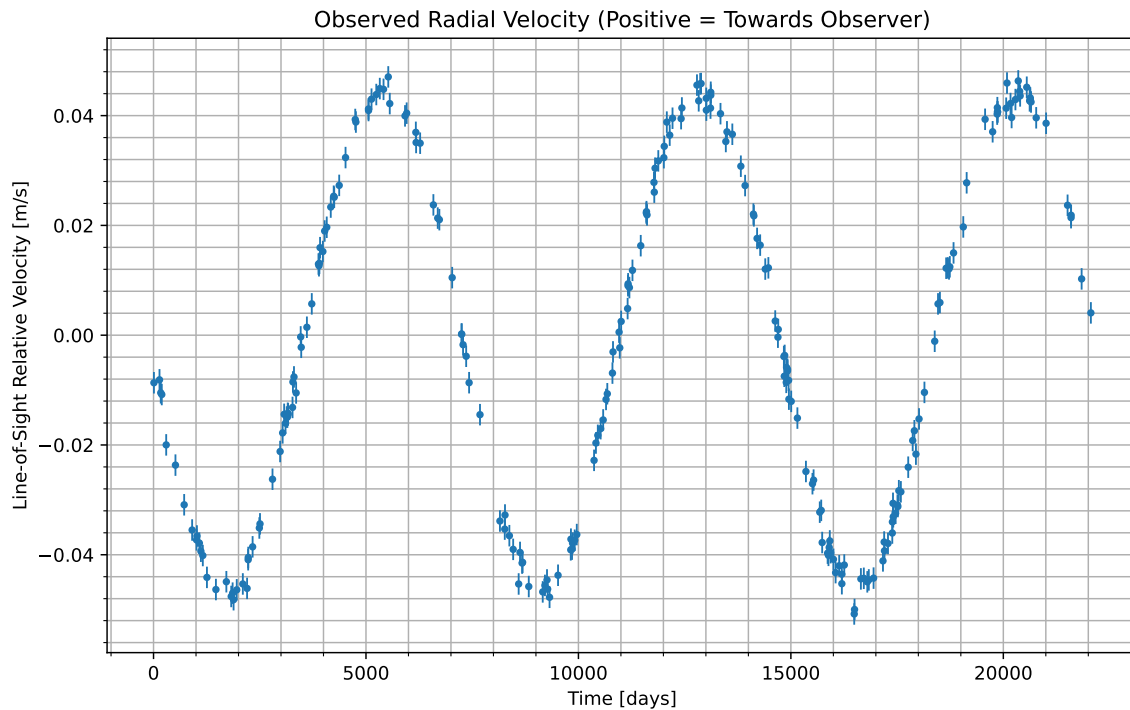
Figure 1: We have isolated the radial velocity of the host star due to the candidate planet. Data begins at UTC 2021-03-18/18:23. Positive values indicate the velocity at which the star is moving towards us; negative indicate the velocity at which it is moving away.
