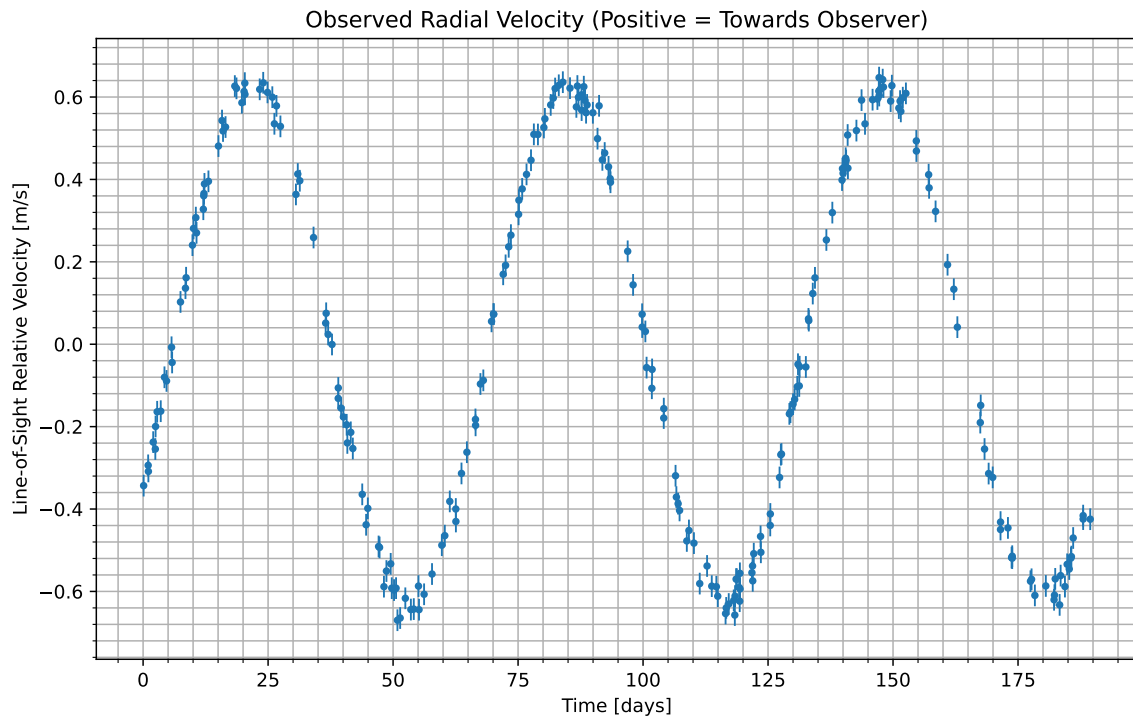
Figure 1: We have isolated the radial velocity of the host star due to the candidate planet. Data begins at UTC 2089-08-16/01:13. Positive values indicate the velocity at which the star is moving towards us; negative indicate the velocity at which it is moving away.
