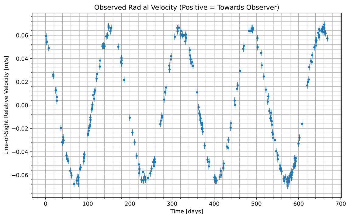
Figure 1: We have isolated the radial velocity of the host star due to the candidate planet. Data begins at UTC 2095-07-01/22:24. Positive values indicate the velocity at which the star is moving towards us; negative indicate the velocity at which it is moving away.
