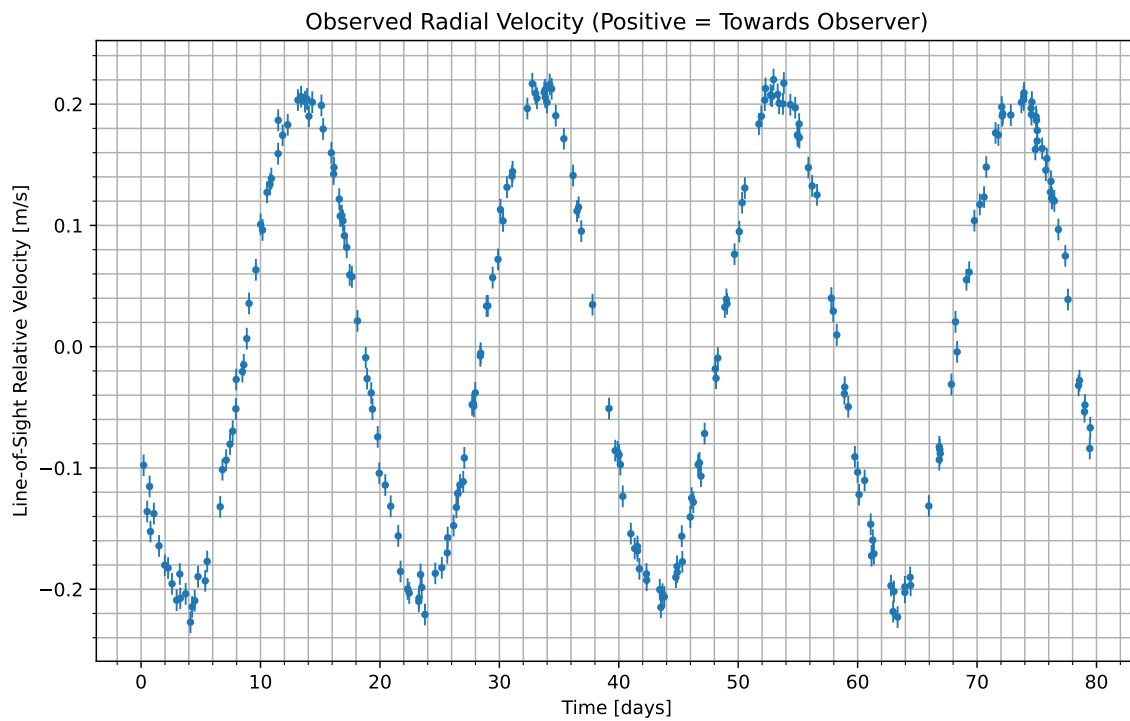
Figure 1: We have isolated the radial velocity of the host star due to the candidate planet. Data begins at UTC 2093-04-17/18:53. Positive values indicate the velocity at which the star is moving towards us; negative indicate the velocity at which it is moving away.
