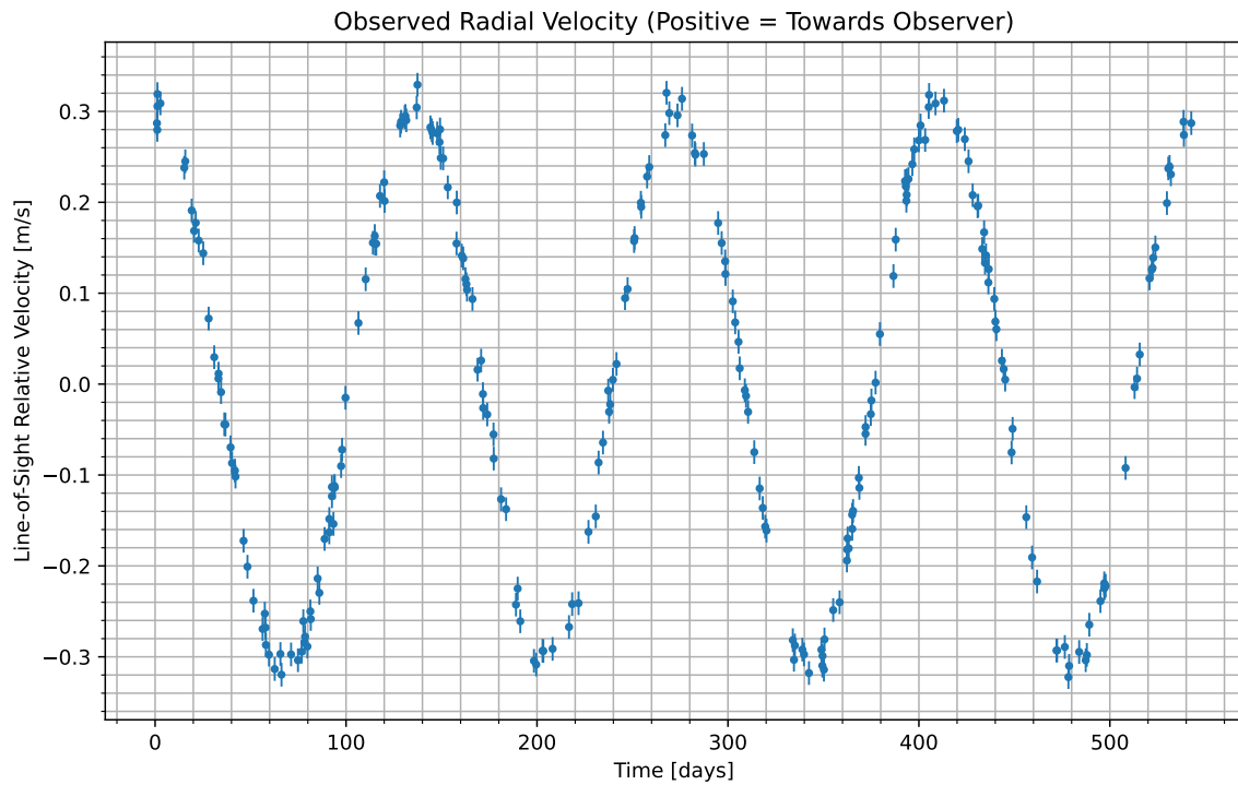
Figure 1: We have isolated the radial velocity of the host star due to the candidate planet. Data begins at UTC 2085-09-11/09:21. Positive values indicate the velocity at which the star is moving towards us; negative indicate the velocity at which it is moving away.
