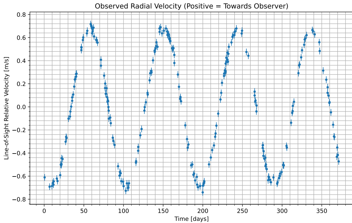
Figure 1: We have isolated the radial velocity of the host star due to the candidate planet. Data begins at UTC 2082-04-03/02:24. Positive values indicate the velocity at which the star is moving towards us; negative indicate the velocity at which it is moving away.
