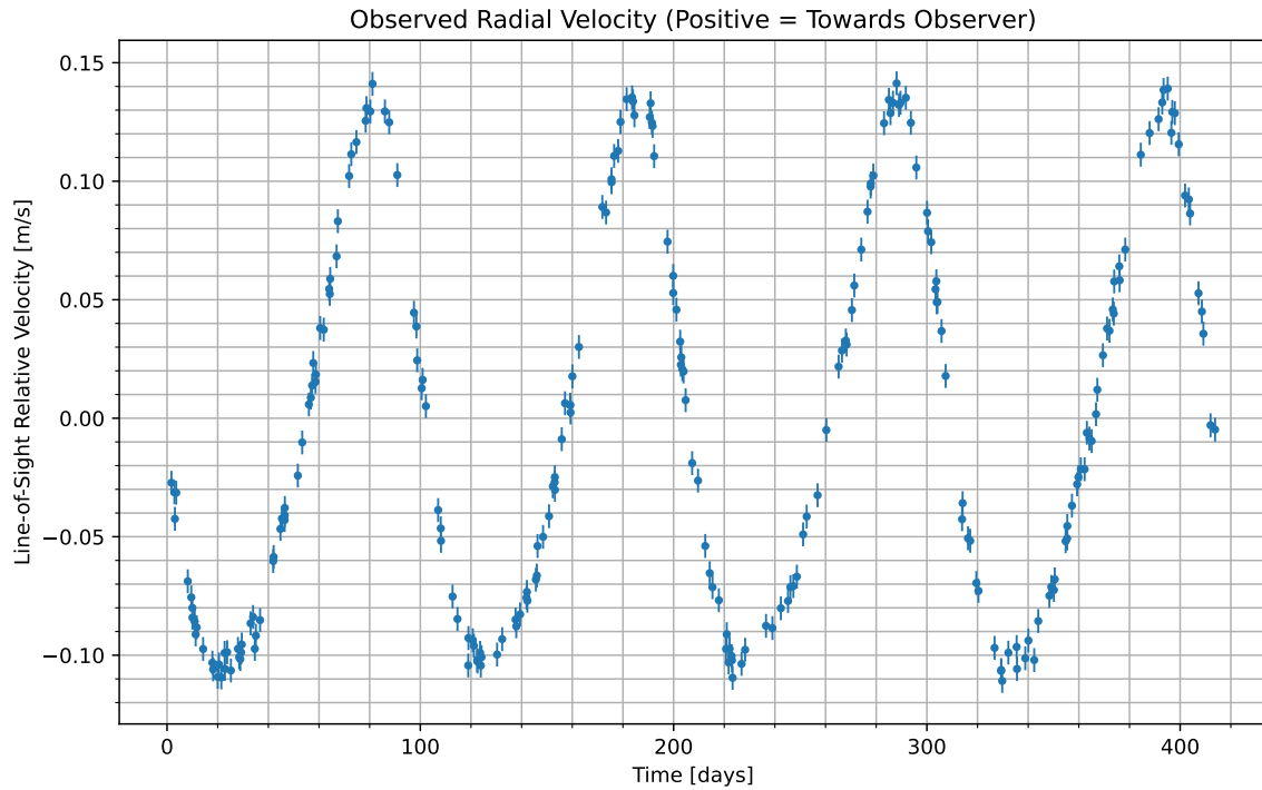
Figure 1: We have isolated the radial velocity of the host star due to the candidate planet. Data begins at UTC 2078-08-31/03:46. Positive values indicate the velocity at which the star is moving towards us; negative indicate the velocity at which it is moving away.
