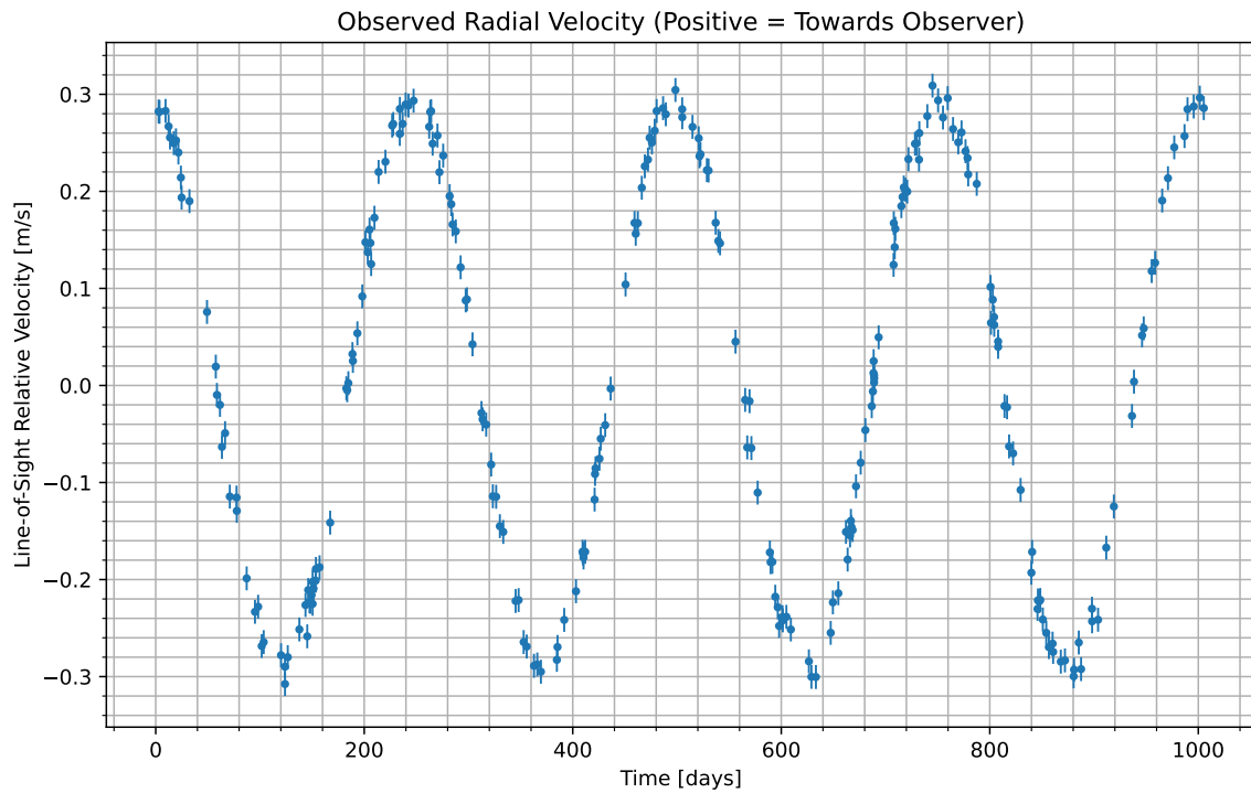
Figure 1: We have isolated the radial velocity of the host star due to the candidate planet. Data begins at UTC 2080-10-27/10:11. Positive values indicate the velocity at which the star is moving towards us; negative indicate the velocity at which it is moving away.
