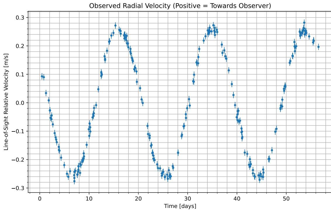
Figure 1: We have isolated the radial velocity of the host star due to the candidate planet. Data begins at UTC 2074-10-22/18:49. Positive values indicate the velocity at which the star is moving towards us; negative indicate the velocity at which it is moving away.
