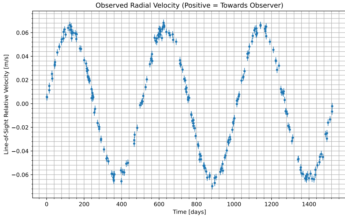
Figure 1: We have isolated the radial velocity of the host star due to the candidate planet. Data begins at UTC 2096-09-23/22:20. Positive values indicate the velocity at which the star is moving towards us; negative indicate the velocity at which it is moving away.
