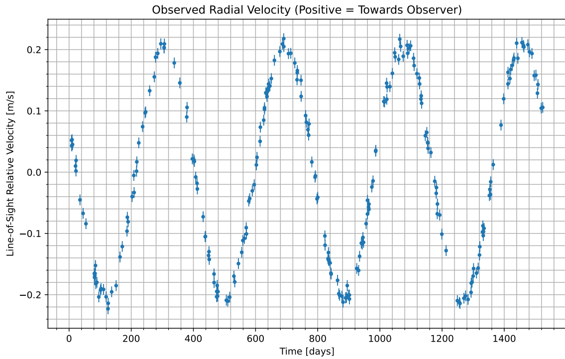
Figure 1: We have isolated the radial velocity of the host star due to the candidate planet. Data begins at UTC 2089-04-19/20:42. Positive values indicate the velocity at which the star is moving towards us; negative indicate the velocity at which it is moving away.
