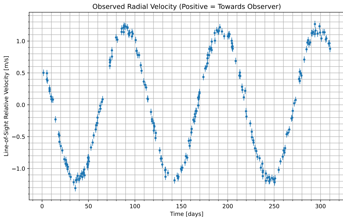
Figure 1: We have isolated the radial velocity of the host star due to the candidate planet. Data begins at UTC 2077-04-21/10:37. Positive values indicate the velocity at which the star is moving towards us; negative indicate the velocity at which it is moving away.
