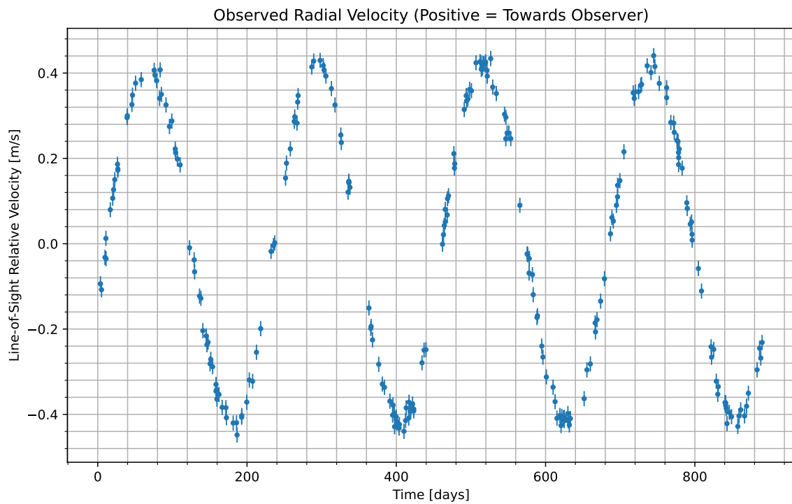
Figure 1: We have isolated the radial velocity of the host star due to the candidate planet. Data begins at UTC 2068-09-24/18:35. Positive values indicate the velocity at which the star is moving towards us; negative indicate the velocity at which it is moving away.
