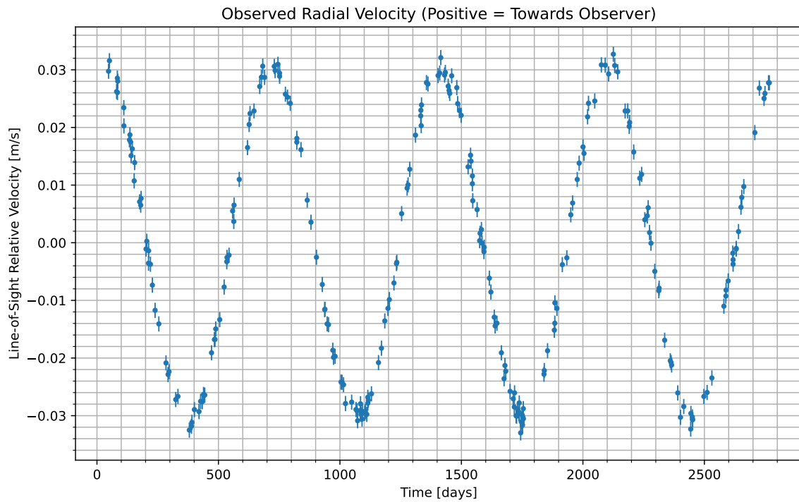
Figure 1: We have isolated the radial velocity of the host star due to the candidate planet. Data begins at UTC 2079-08-05/15:43. Positive values indicate the velocity at which the star is moving towards us; negative indicate the velocity at which it is moving away.
