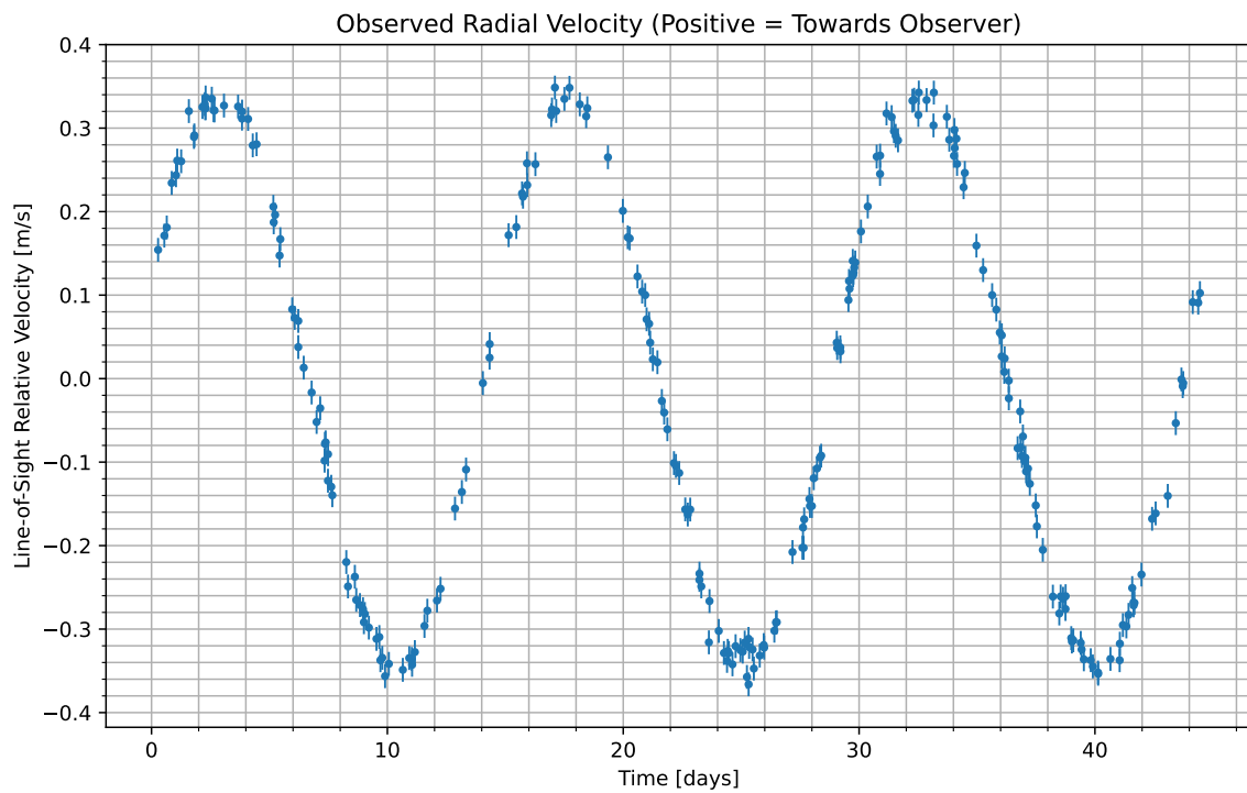
Figure 1: We have isolated the radial velocity of the host star due to the candidate planet. Data begins at UTC 2095-01-13/16:07. Positive values indicate the velocity at which the star is moving towards us; negative indicate the velocity at which it is moving away.
