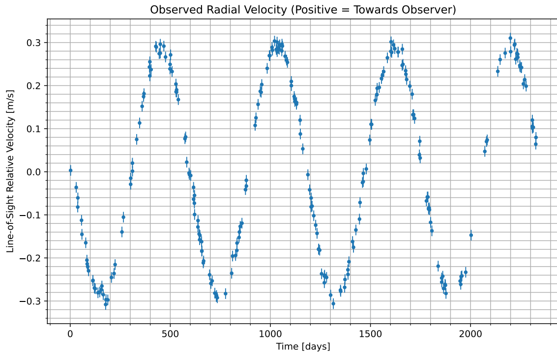
Figure 1: We have isolated the radial velocity of the host star due to the candidate planet. Data begins at UTC 2067-04-26/21:46. Positive values indicate the velocity at which the star is moving towards us; negative indicate the velocity at which it is moving away.
