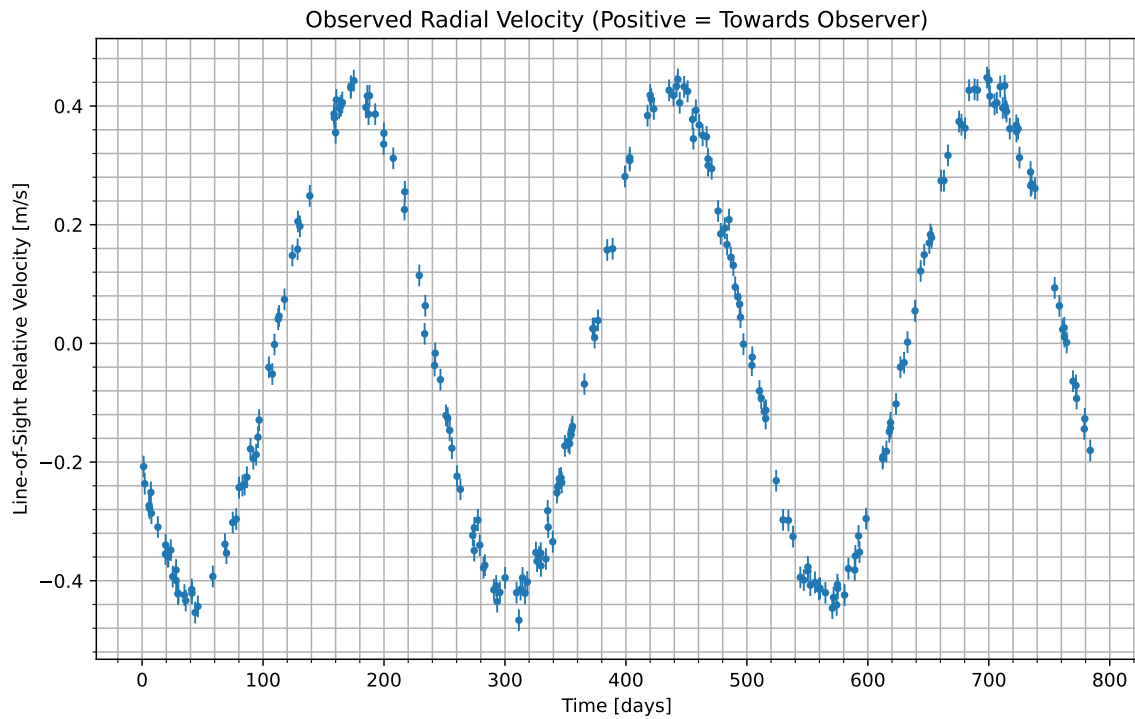
Figure 1: We have isolated the radial velocity of the host star due to the candidate planet. Data begins at UTC 2078-12-13/19:41. Positive values indicate the velocity at which the star is moving towards us; negative indicate the velocity at which it is moving away.
