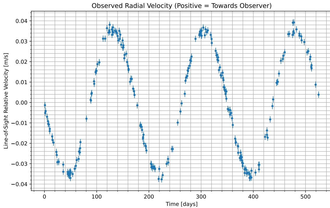
Figure 1: We have isolated the radial velocity of the host star due to the candidate planet. Data begins at UTC 2090-03-02/15:13. Positive values indicate the velocity at which the star is moving towards us; negative indicate the velocity at which it is moving away.
