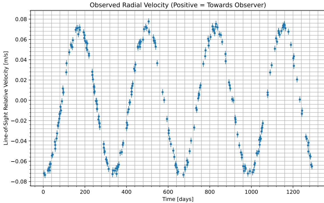
Figure 1: We have isolated the radial velocity of the host star due to the candidate planet. Data begins at UTC 2085-07-12/16:53. Positive values indicate the velocity at which the star is moving towards us; negative indicate the velocity at which it is moving away.
