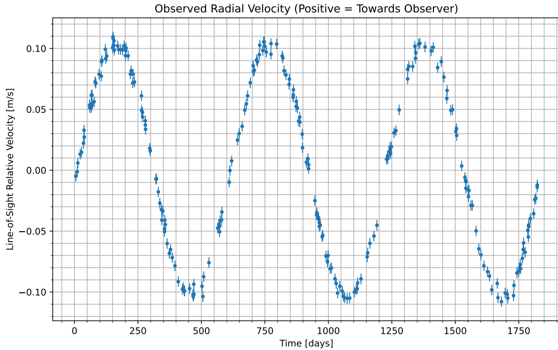
Figure 1: We have isolated the radial velocity of the host star due to the candidate planet. Data begins at UTC 2073-08-30/00:21. Positive values indicate the velocity at which the star is moving towards us; negative indicate the velocity at which it is moving away.
