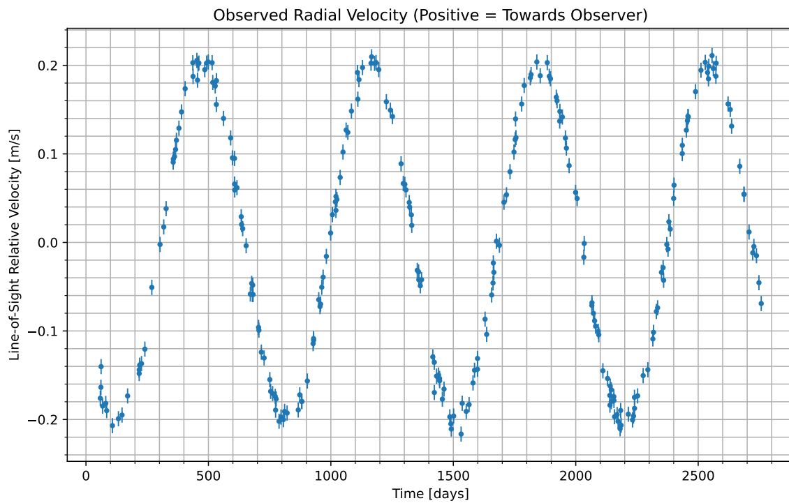
Figure 1: We have isolated the radial velocity of the host star due to the candidate planet. Data begins at UTC 2068-07-15/13:40. Positive values indicate the velocity at which the star is moving towards us; negative indicate the velocity at which it is moving away.
