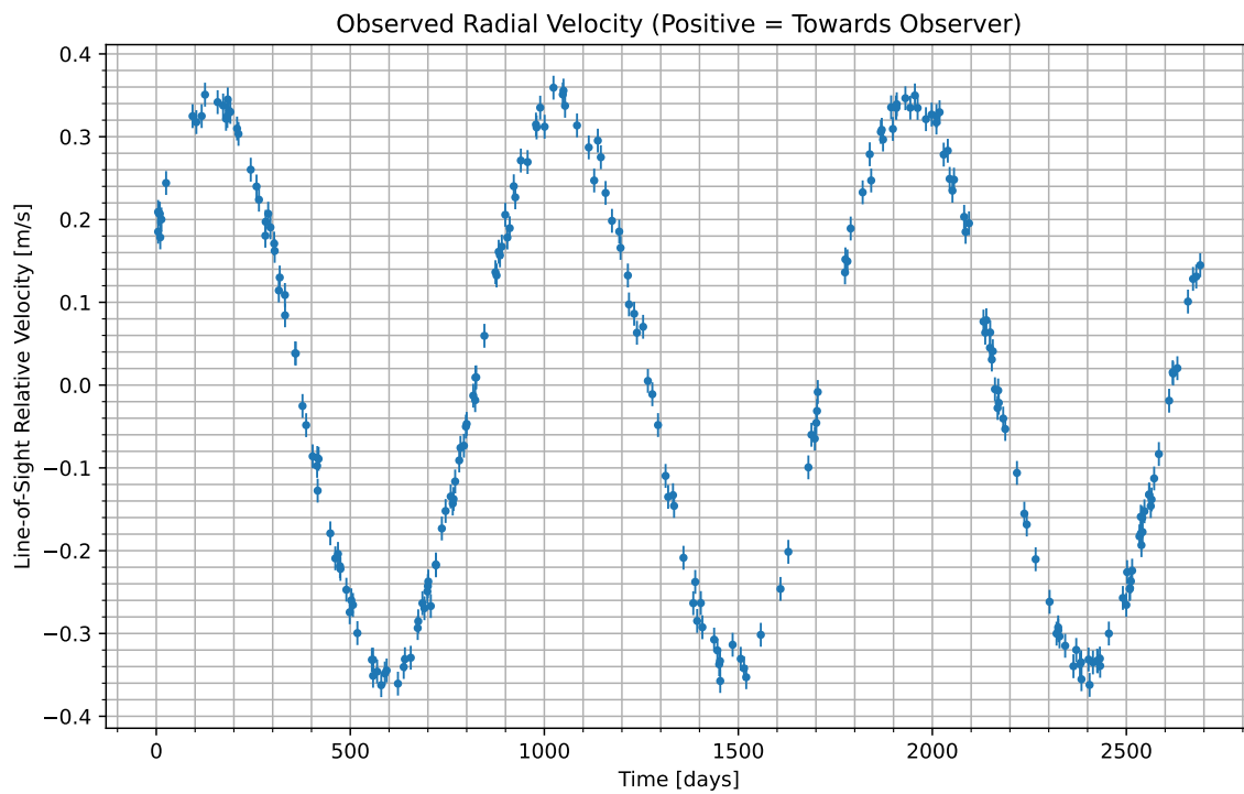
Figure 1: We have isolated the radial velocity of the host star due to the candidate planet. Data begins at UTC 2068-08-01/18:27. Positive values indicate the velocity at which the star is moving towards us; negative indicate the velocity at which it is moving away.
