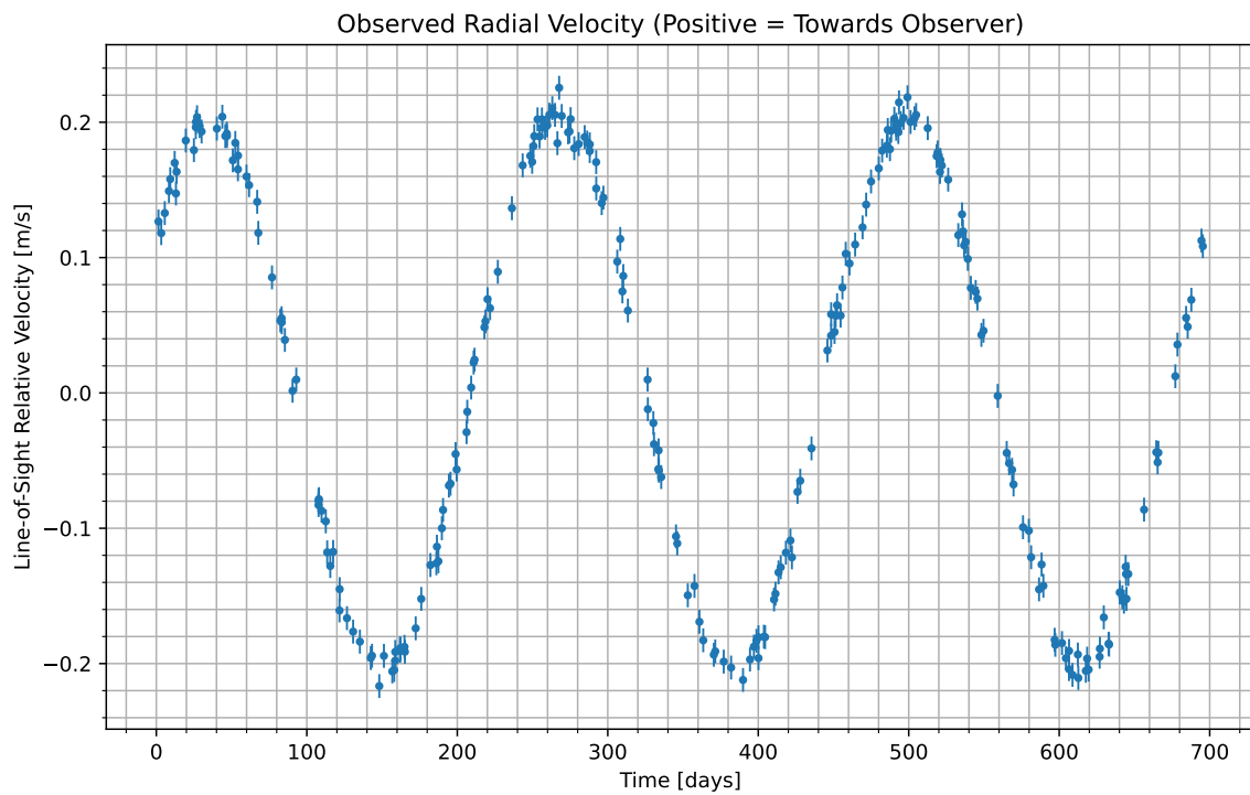
Figure 1: We have isolated the radial velocity of the host star due to the candidate planet. Data begins at UTC 2083-11-15/17:58. Positive values indicate the velocity at which the star is moving towards us; negative indicate the velocity at which it is moving away.
