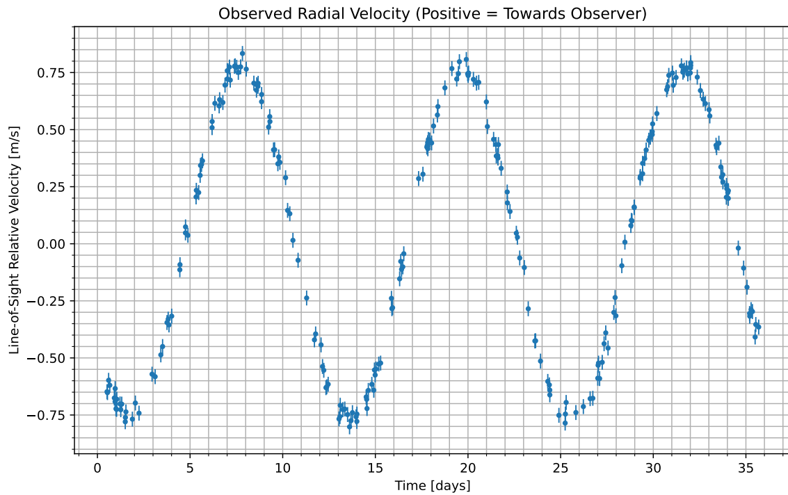
Figure 1: We have isolated the radial velocity of the host star due to the candidate planet. Data begins at UTC 2089-07-01/19:45. Positive values indicate the velocity at which the star is moving towards us; negative indicate the velocity at which it is moving away.
