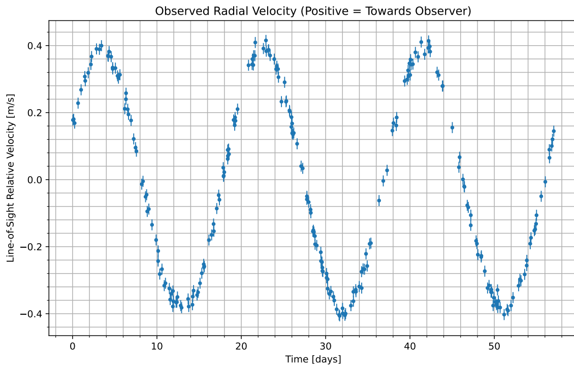
Figure 1: We have isolated the radial velocity of the host star due to the candidate planet. Data begins at UTC 2076-06-07/18:15. Positive values indicate the velocity at which the star is moving towards us; negative indicate the velocity at which it is moving away.
