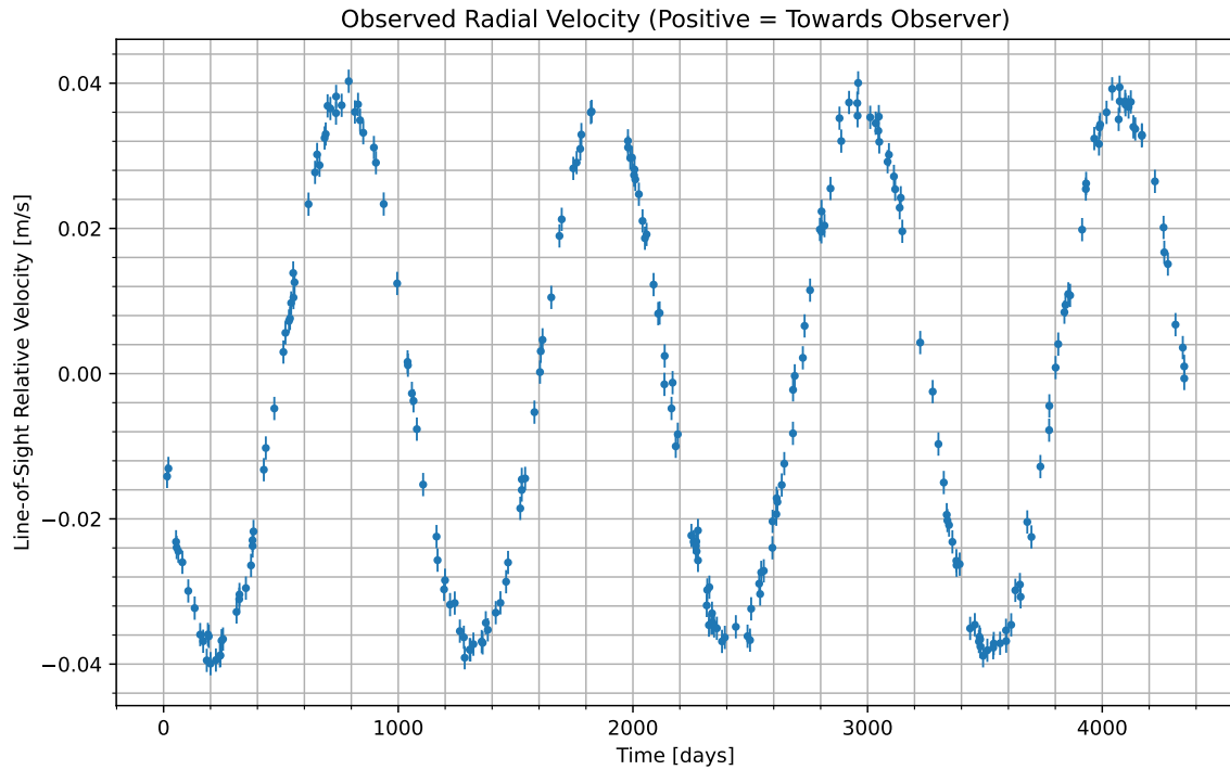
Figure 1: We have isolated the radial velocity of the host star due to the candidate planet. Data begins at UTC 2078-11-09/23:31. Positive values indicate the velocity at which the star is moving towards us; negative indicate the velocity at which it is moving away.
