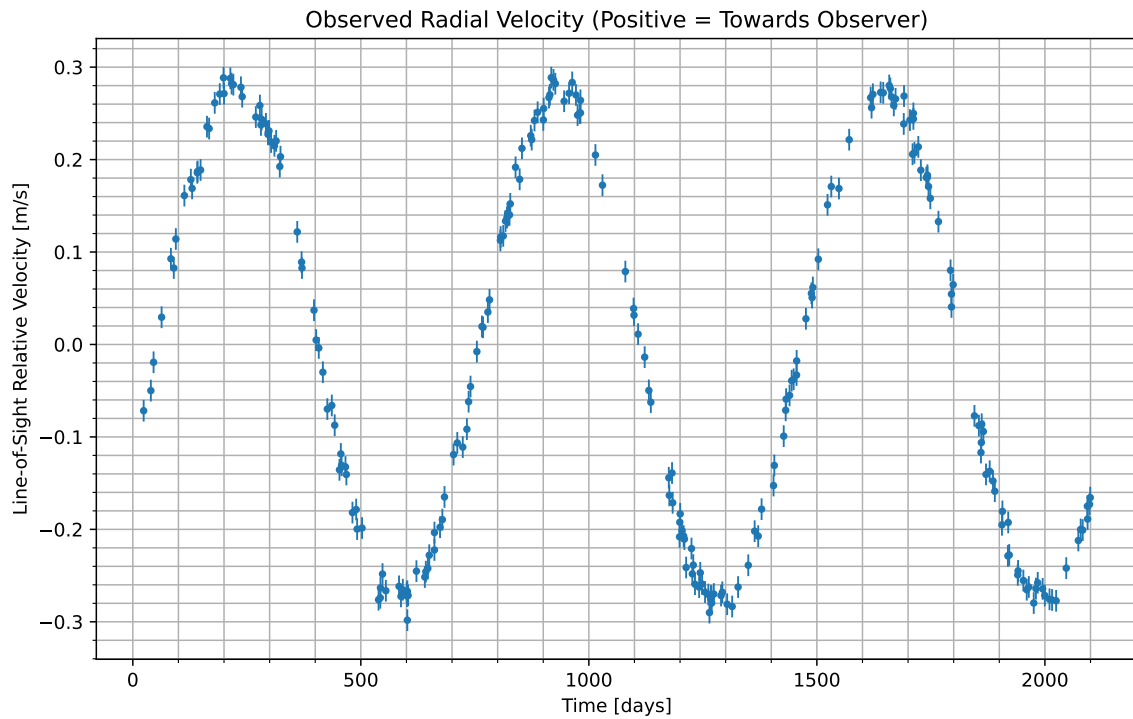
Figure 1: We have isolated the radial velocity of the host star due to the candidate planet. Data begins at UTC 2080-01-28/14:54. Positive values indicate the velocity at which the star is moving towards us; negative indicate the velocity at which it is moving away.
