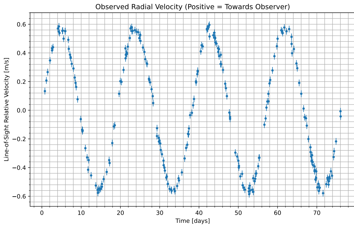
Figure 1: We have isolated the radial velocity of the host star due to the candidate planet. Data begins at UTC 2096-12-07/04:48. Positive values indicate the velocity at which the star is moving towards us; negative indicate the velocity at which it is moving away.
