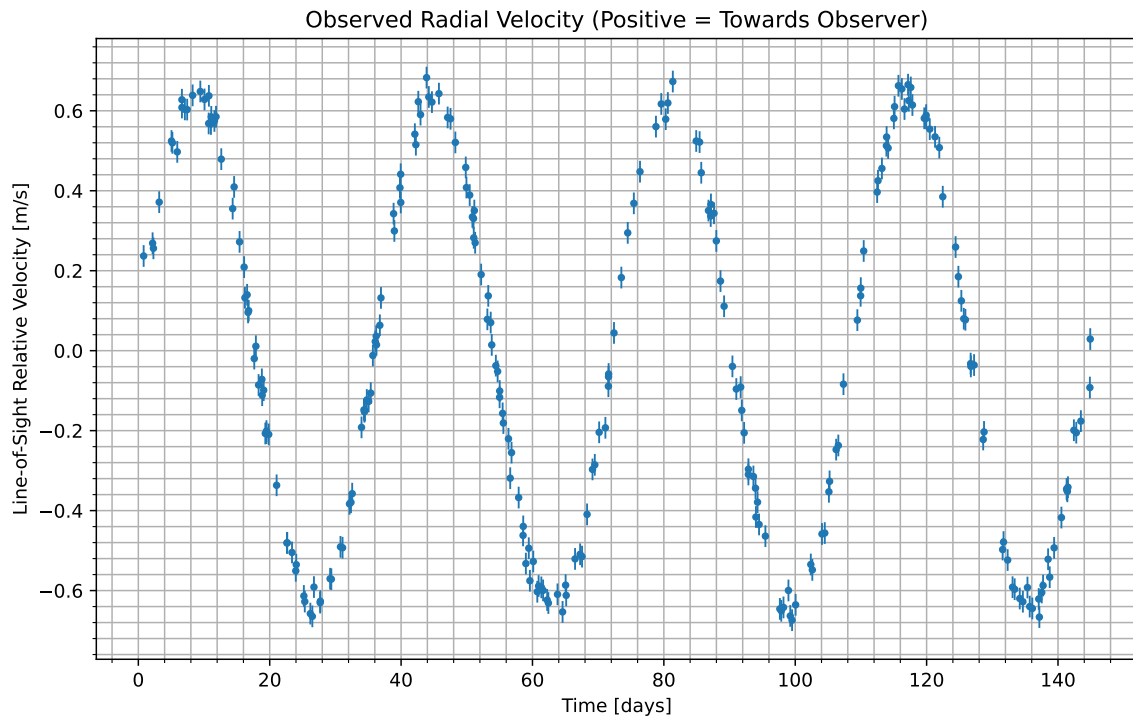
Figure 1: We have isolated the radial velocity of the host star due to the candidate planet. Data begins at UTC 2096-11-04/02:16. Positive values indicate the velocity at which the star is moving towards us; negative indicate the velocity at which it is moving away.
