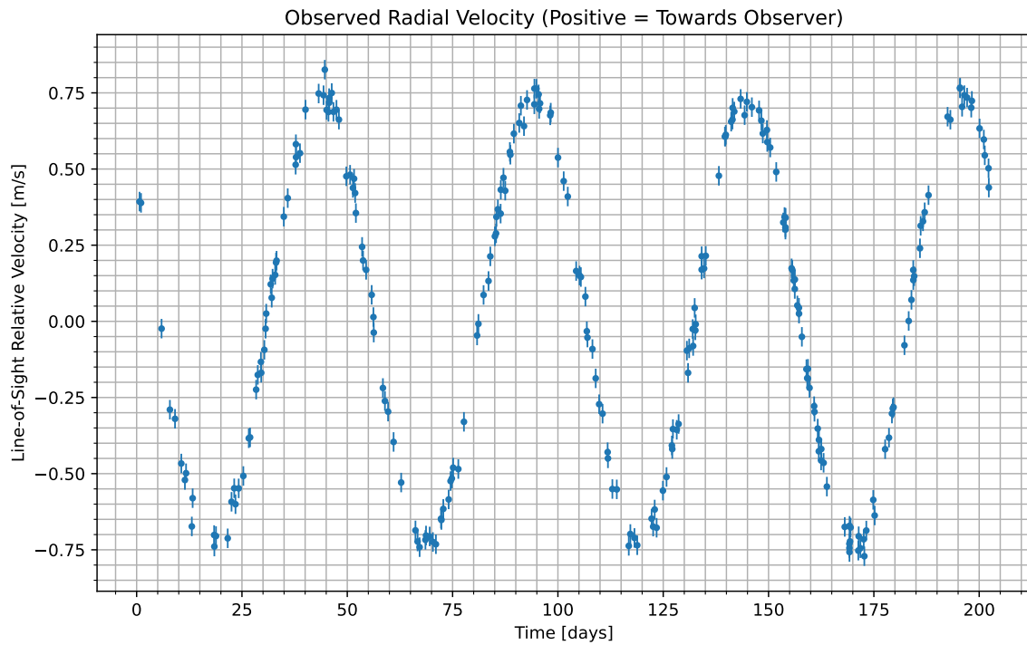
Figure 1: We have isolated the radial velocity of the host star due to the candidate planet. Data begins at UTC 2082-07-20/03:17. Positive values indicate the velocity at which the star is moving towards us; negative indicate the velocity at which it is moving away.
