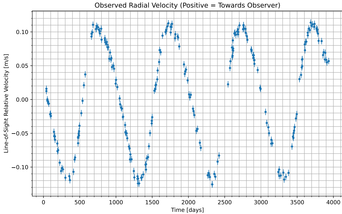
Figure 1: We have isolated the radial velocity of the host star due to the candidate planet. Data begins at UTC 2078-09-22/18:10. Positive values indicate the velocity at which the star is moving towards us; negative indicate the velocity at which it is moving away.
