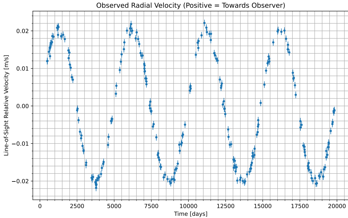
Figure 1: We have isolated the radial velocity of the host star due to the candidate planet. Data begins at UTC 2027-09-25/21:11. Positive values indicate the velocity at which the star is moving towards us; negative indicate the velocity at which it is moving away.
