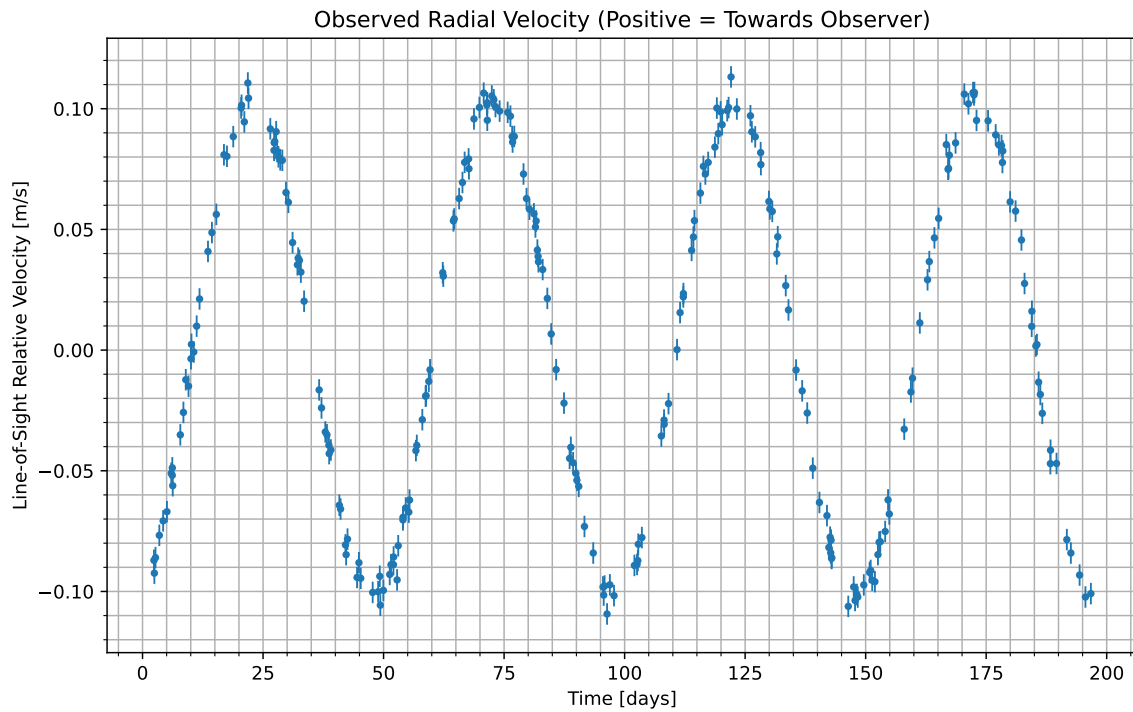
Figure 1: We have isolated the radial velocity of the host star due to the candidate planet. Data begins at UTC 2086-08-01/17:02. Positive values indicate the velocity at which the star is moving towards us; negative indicate the velocity at which it is moving away.
