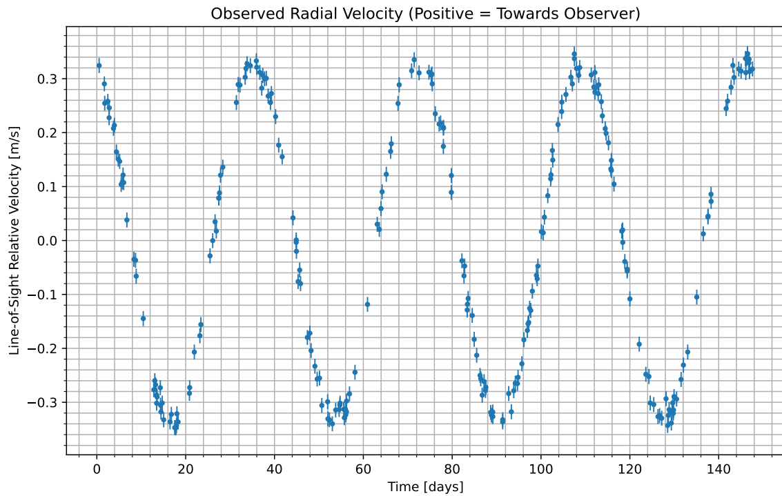
Figure 1: We have isolated the radial velocity of the host star due to the candidate planet. Data begins at UTC 2078-01-18/11:16. Positive values indicate the velocity at which the star is moving towards us; negative indicate the velocity at which it is moving away.
