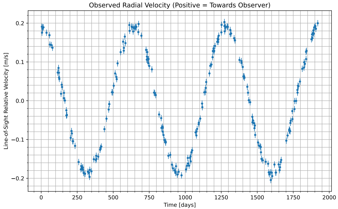
Figure 1: We have isolated the radial velocity of the host star due to the candidate planet. Data begins at UTC 2069-04-27/19:14. Positive values indicate the velocity at which the star is moving towards us; negative indicate the velocity at which it is moving away.
