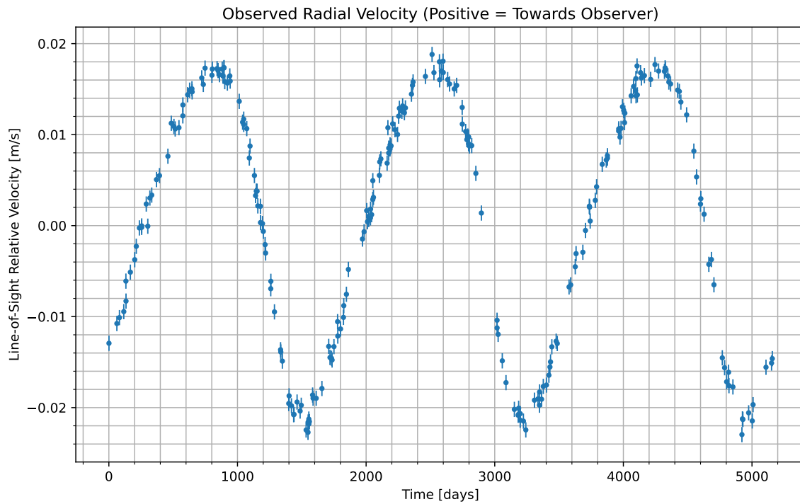
Figure 1: We have isolated the radial velocity of the host star due to the candidate planet. Data begins at UTC 2058-11-18/18:10. Positive values indicate the velocity at which the star is moving towards us; negative indicate the velocity at which it is moving away.
