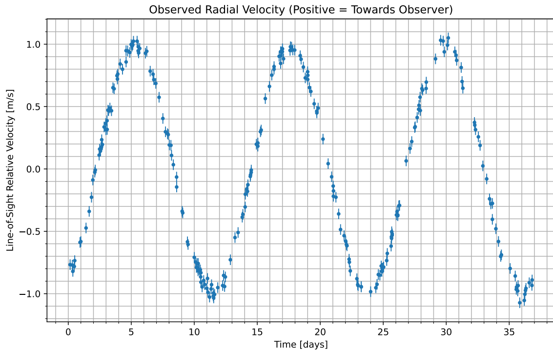
Figure 1: We have isolated the radial velocity of the host star due to the candidate planet. Data begins at UTC 2080-05-16/07:04. Positive values indicate the velocity at which the star is moving towards us; negative indicate the velocity at which it is moving away.
