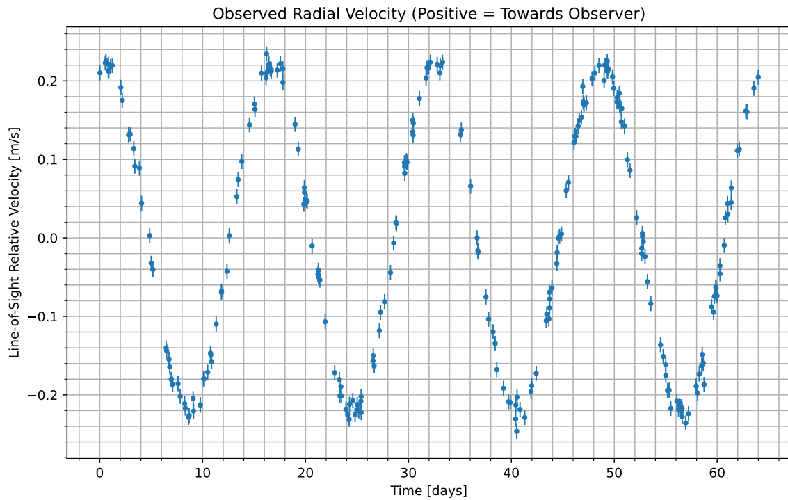
Figure 1: We have isolated the radial velocity of the host star due to the candidate planet. Data begins at UTC 2072-01-06/06:40. Positive values indicate the velocity at which the star is moving towards us; negative indicate the velocity at which it is moving away.
